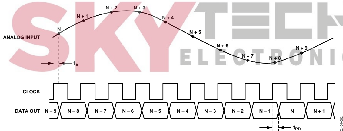
Figure 2. Input Timing
