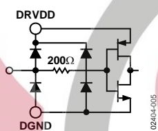
Figure 5. Three-State (OEB)
