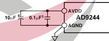
Figure 61. Analog Supply Decoupling
