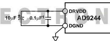
Figure 62. Digital Supply Decoupling
