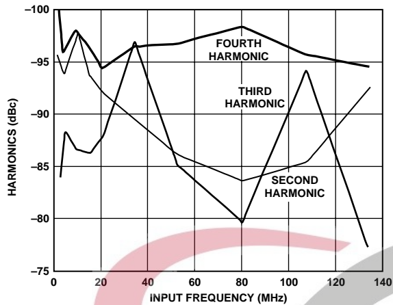
Figure 22. Harmonics vs. Input Frequency
