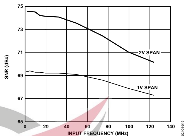
Figure 19. SNR vs. Input Frequency
