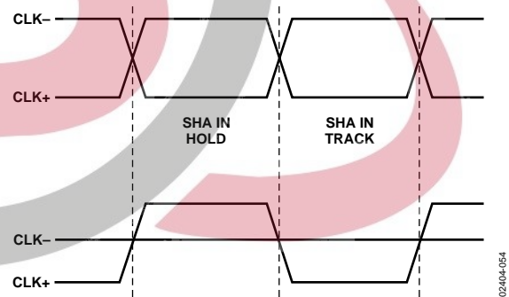
Figure 54. SHA Timing
