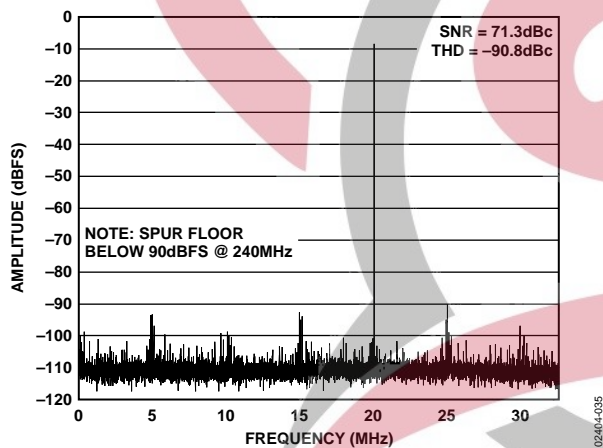
Figure 35. Driving ADC Inputs with Transformer and Balun, f_{IN} = 240 MHz, A_{IN} = -8.5 dBFS
